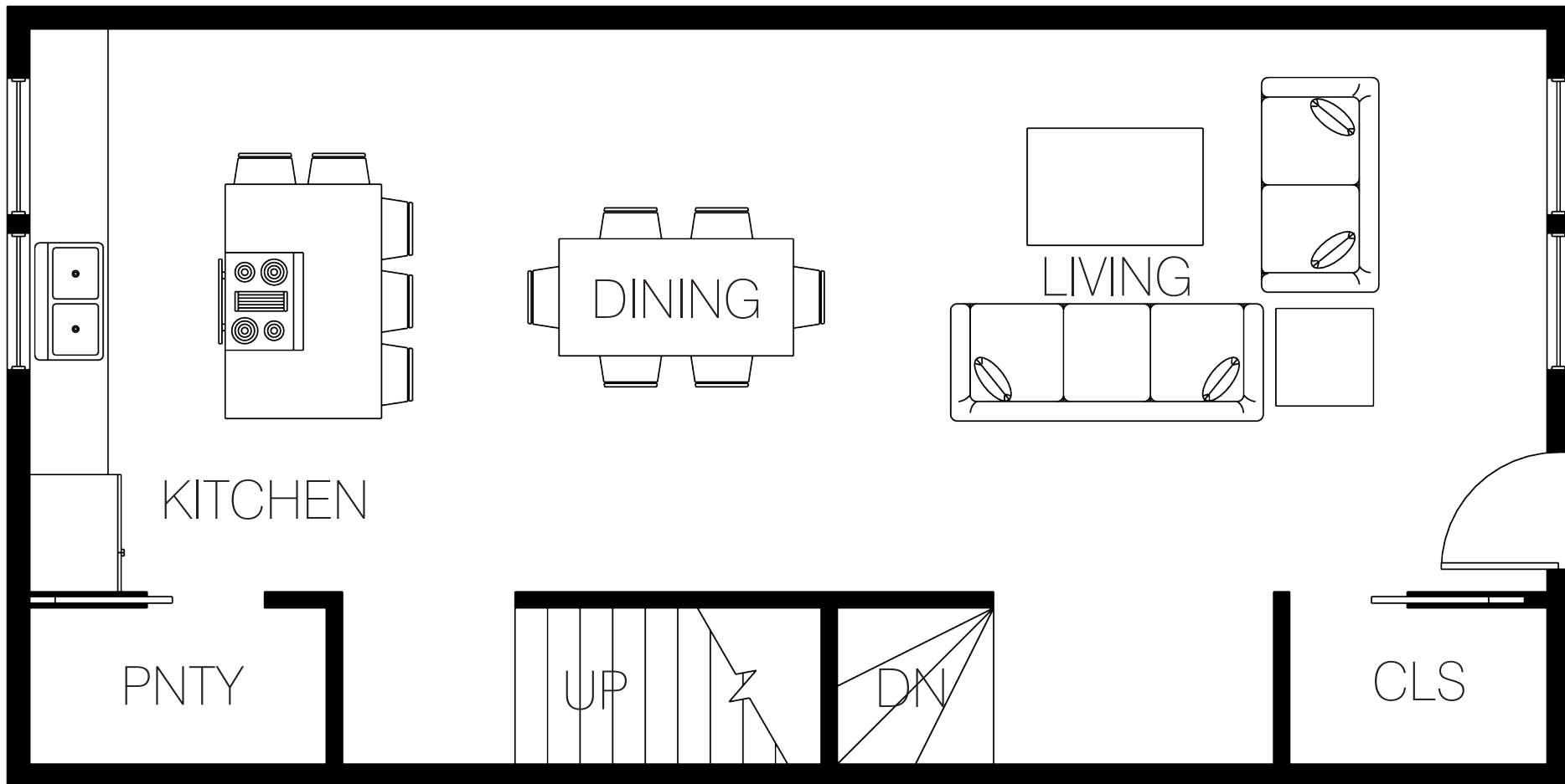
Level 1 1/4" = 1'
