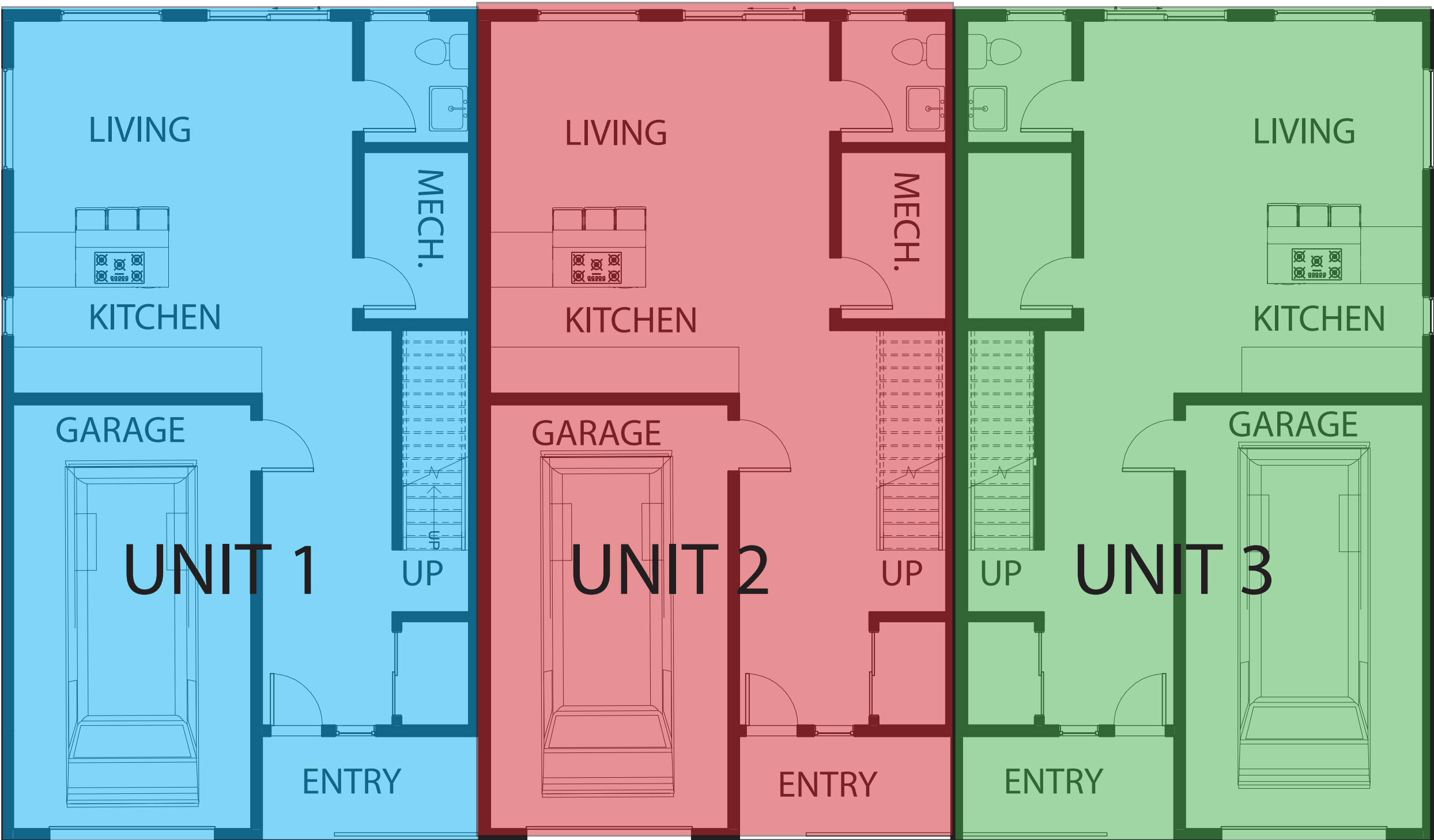
First Floor Plan 3/16" = 1'
