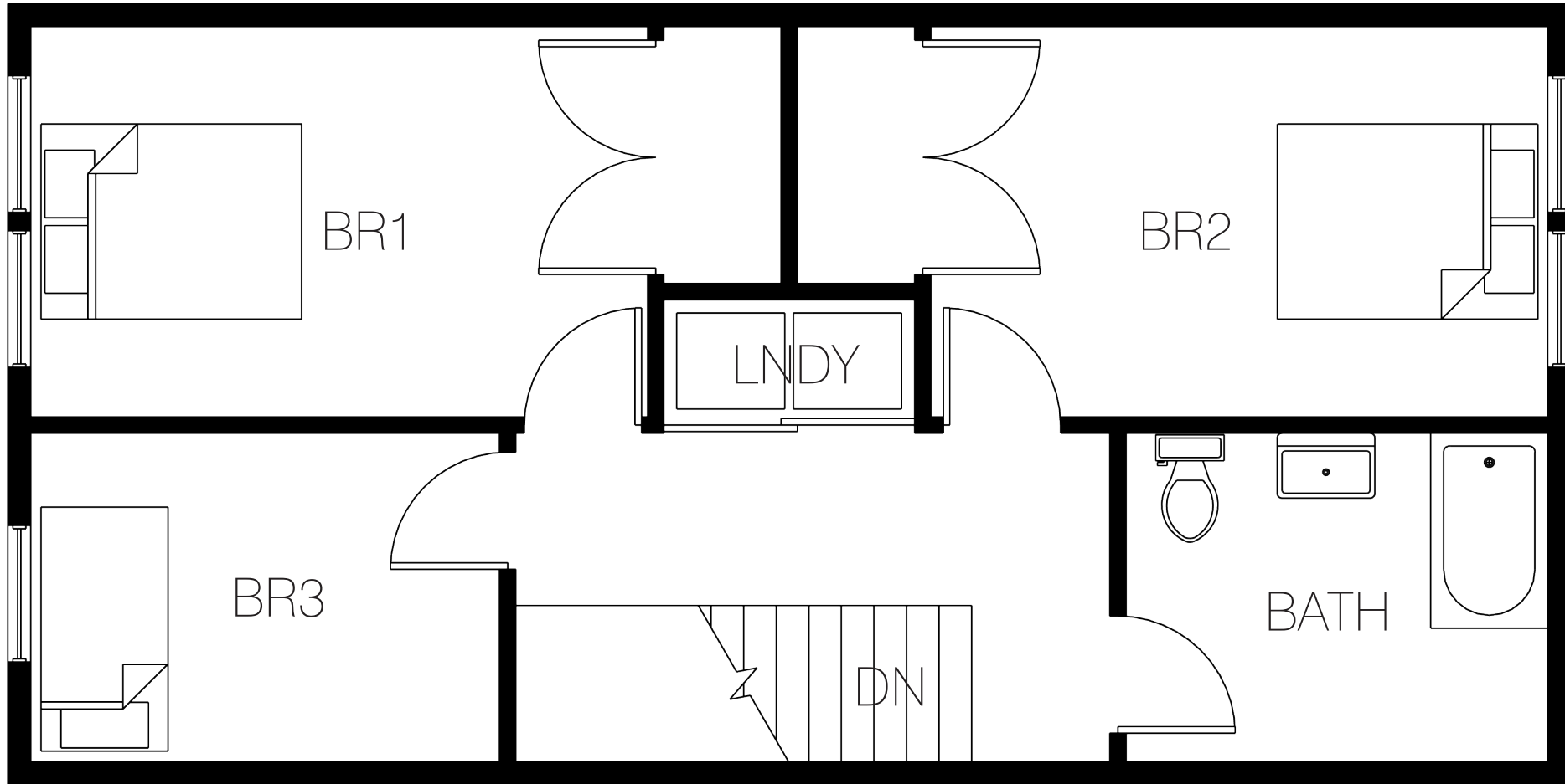
Level 2 1/4" = 1'
