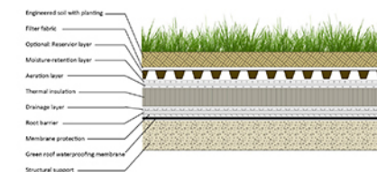
GREEN ROOF ASSEMBLY DIAGRAM
