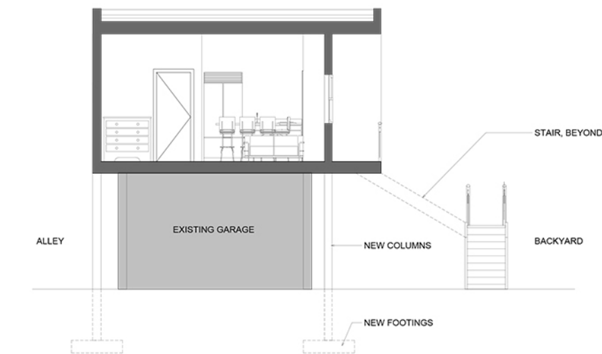
BUILDING SECTION - CONCEPT A - GREEN ROOF
