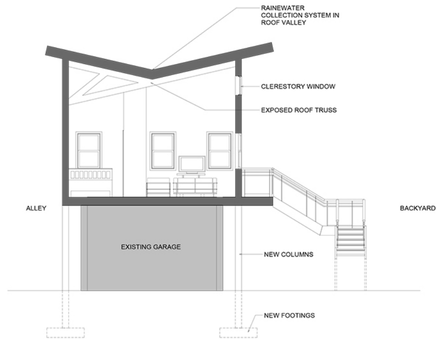
BUILDING SECTION - CONCEPT C - BUTTERFLY ROOF
