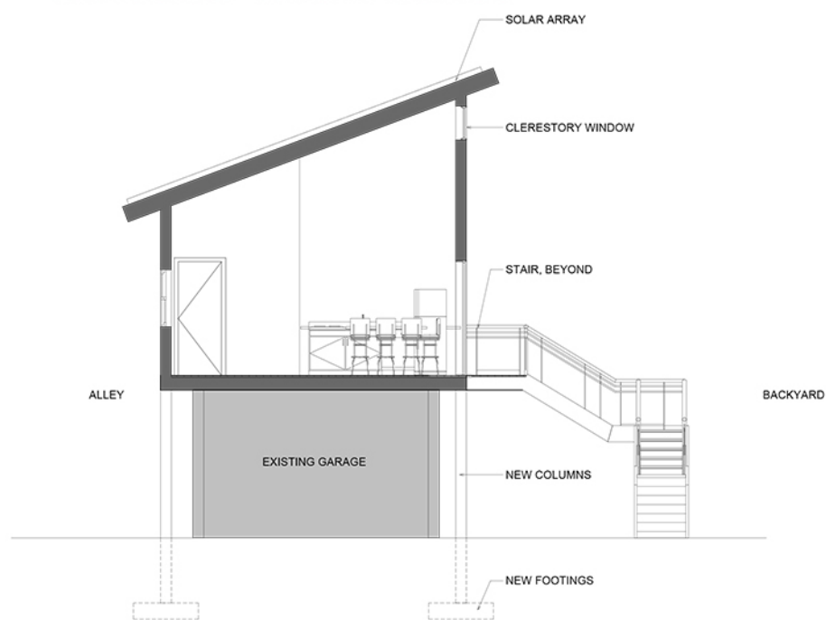
BUILDING SECTION - CONCEPT B - SOLAR CANOPY ROOF
