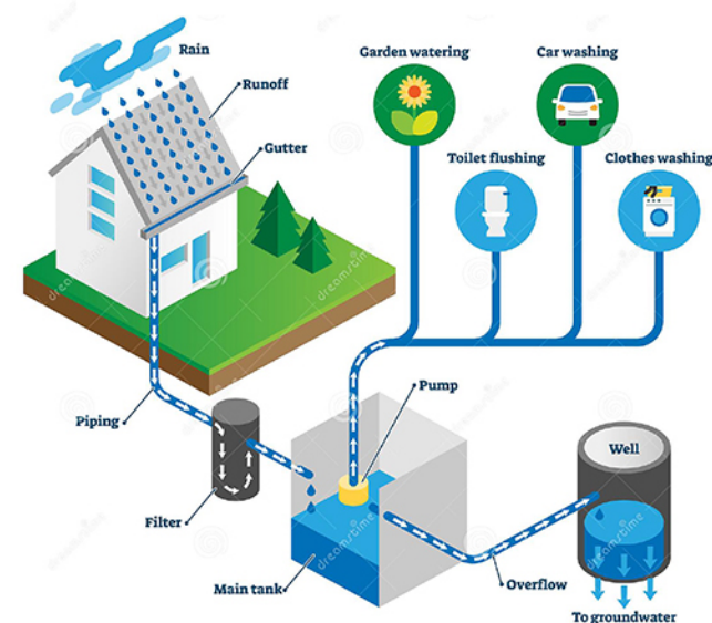
RAINWATER HARVESTING
